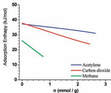
Figure 5. The heat of adsorption of the activated 1 for acetylene (blue), carbon dioxide (red), and methane (green).
